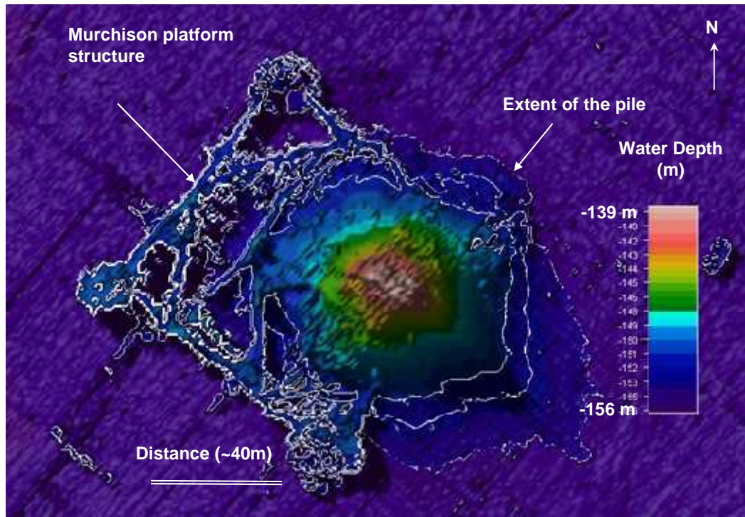
Figure 27: MBES Survey Data of the Murchison Drill Cuttings Pile
