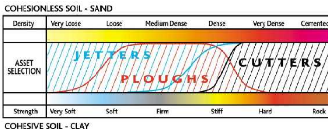
Figure 35: Trenching Equipment V Soil Type
