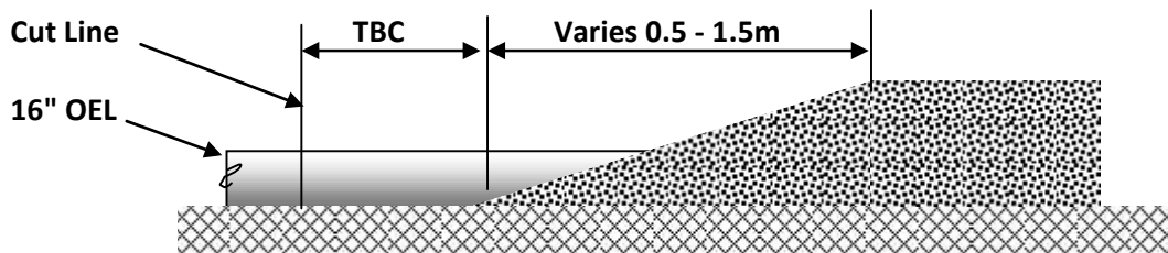
Figure 45: Location of Cut Lines in PL115
