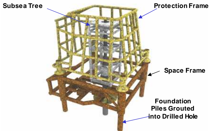
Figure 24: 211/19-2 Subsea Installation
