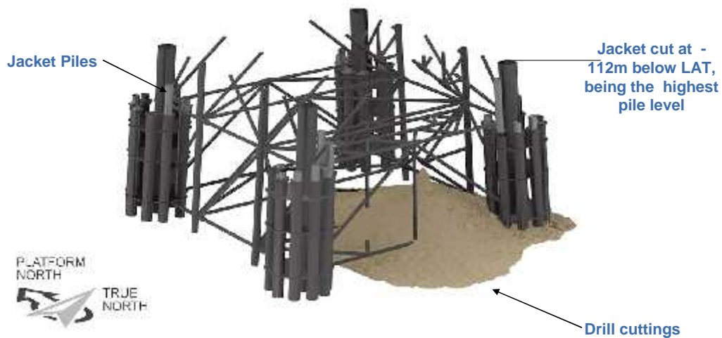
Figure 39: Option 2 - Murchison Jacket Partial Removed
