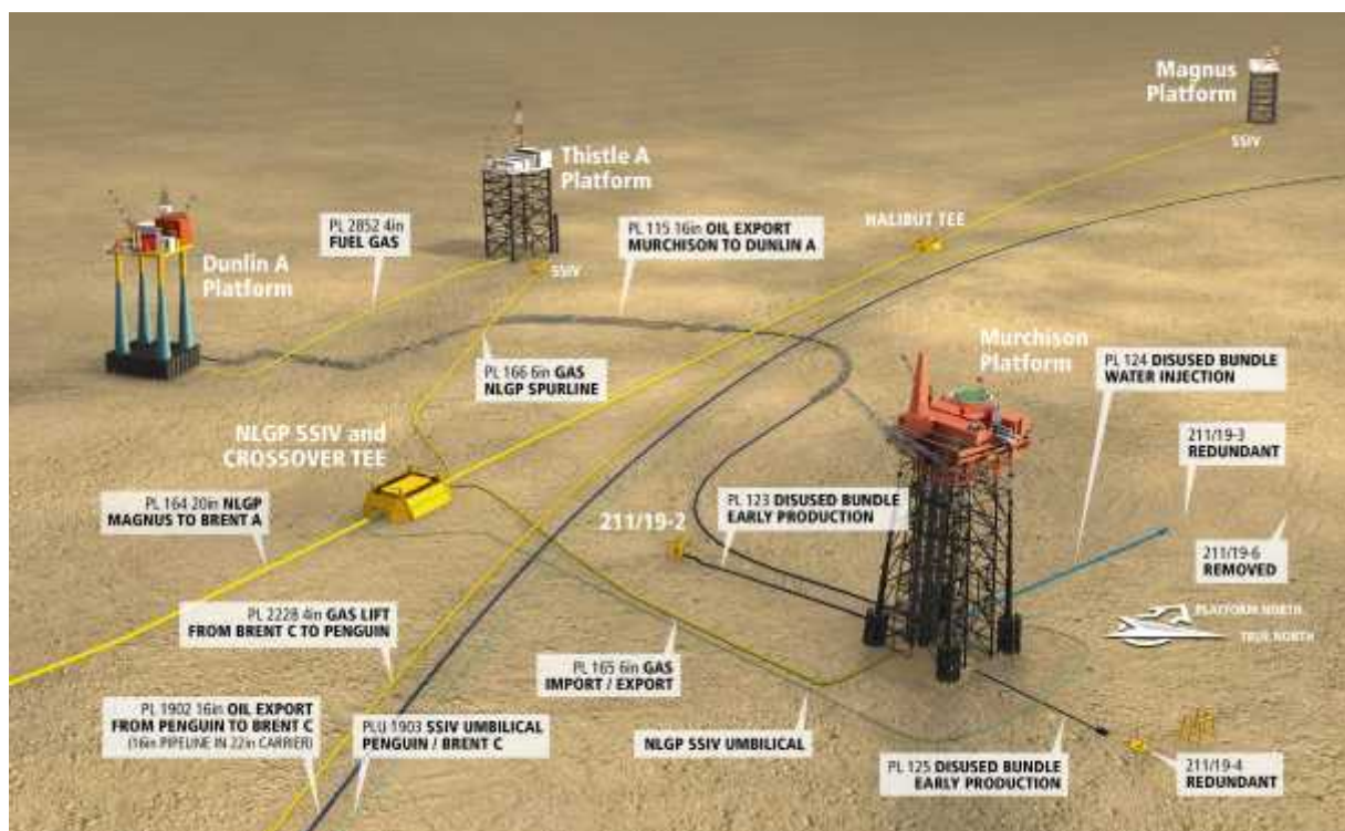
Figure 18: Murchison Subsea Infrastructure
