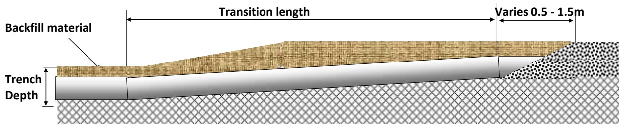
Figure 46: Transition from Rock Placement to Trench 80
