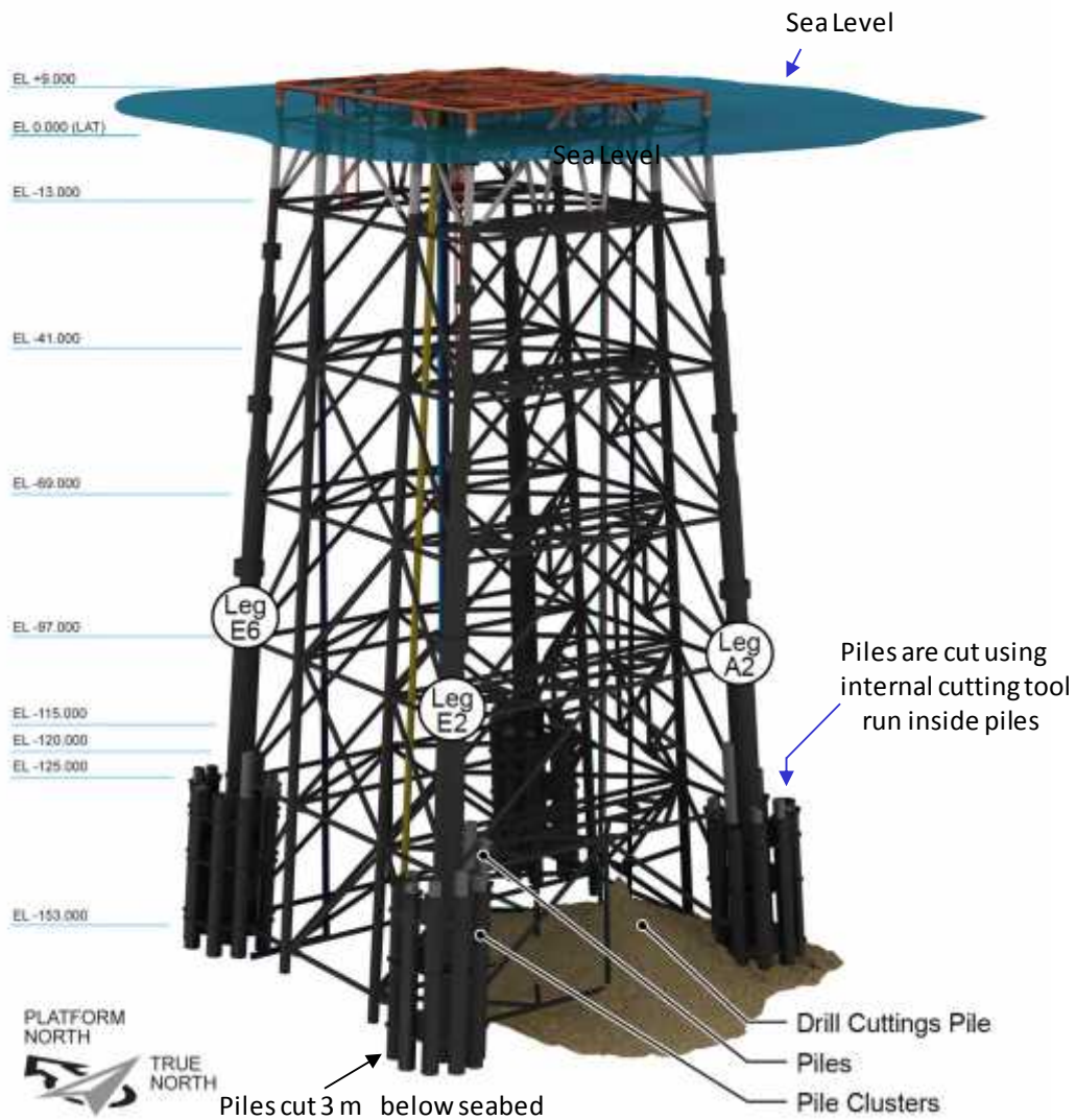
Figure 38: Option 1 -Murchison Jacket Full removal
