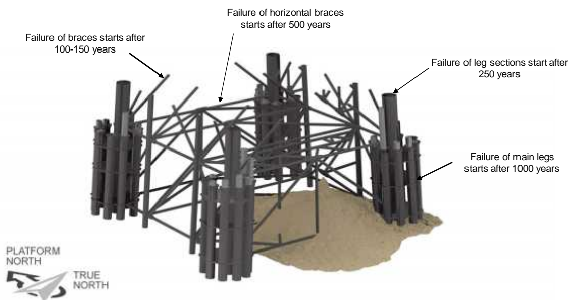
Figure 40: Predicted Degradation Rate of Footings
