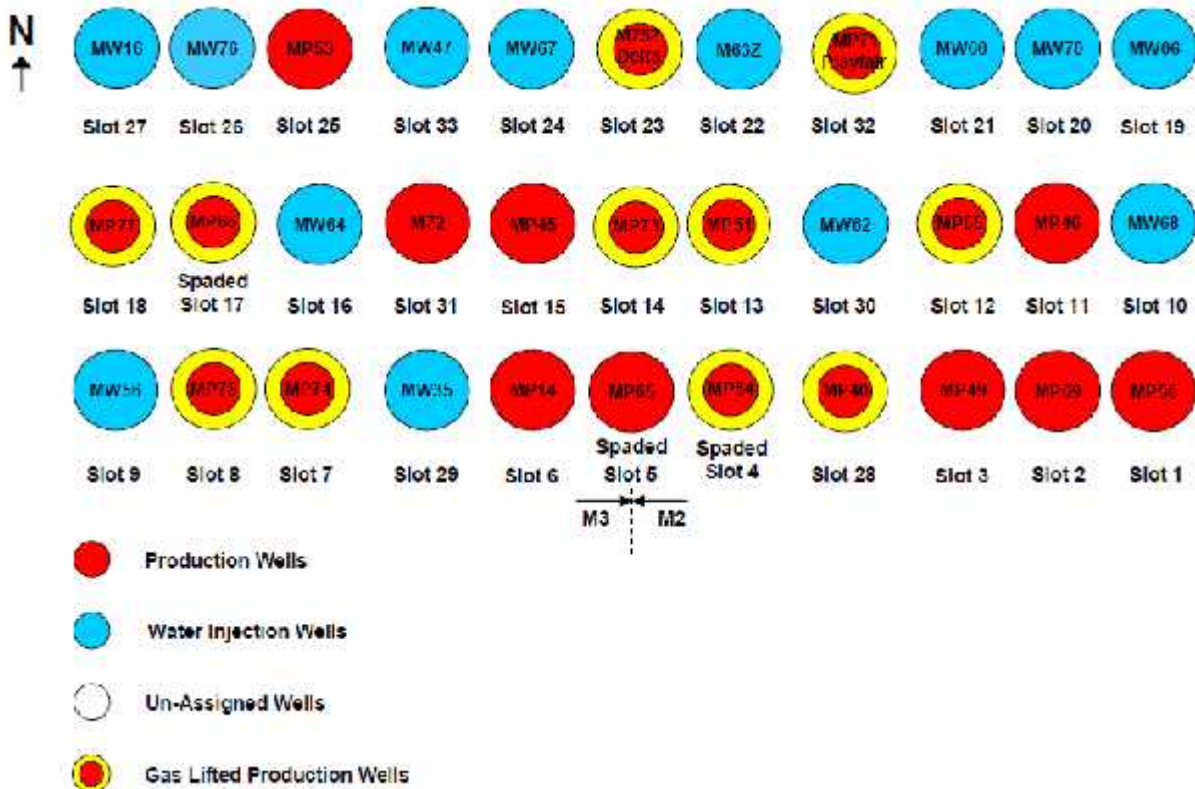
Figure 25: Murchison Well Slot Diagram
