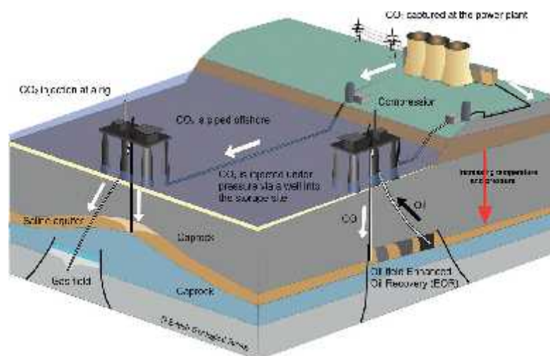
Figure 34: CCS Schematic
