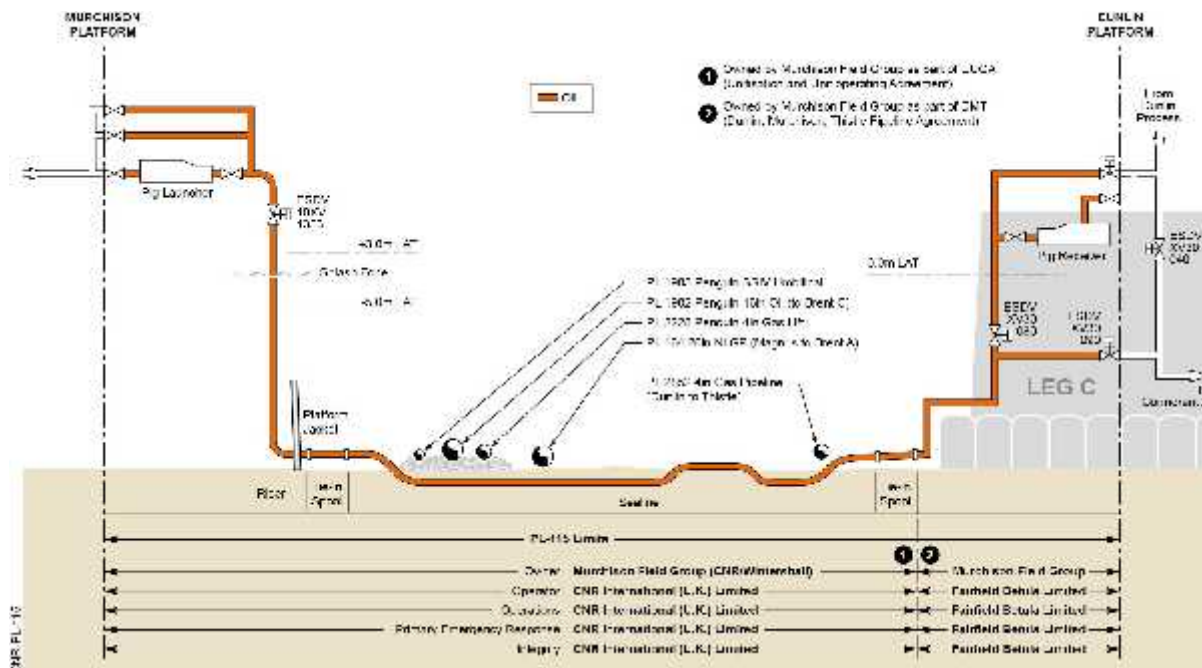
Figure 22: PL115 Schematic
