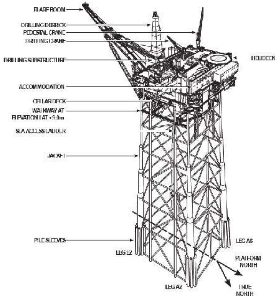
Figure 3: Murchison Platform Components
