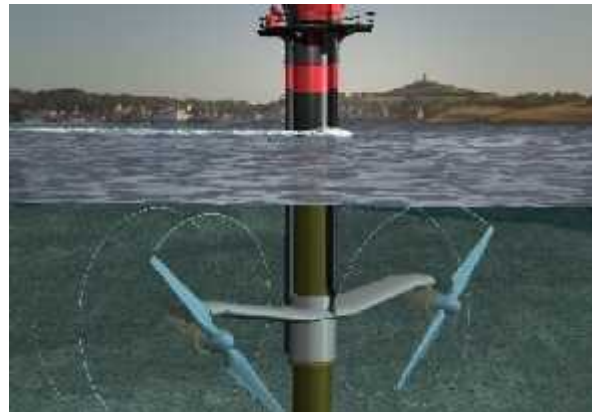
Figure 32: Seagen Drive
