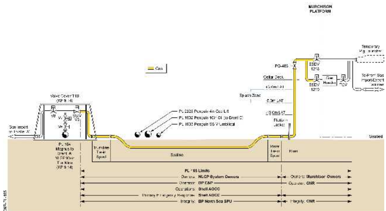
Figure 23: PL165 Schematic
